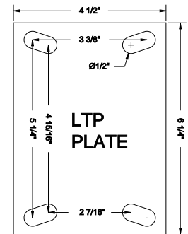
STANDARD TOP PLATE (LTP)
